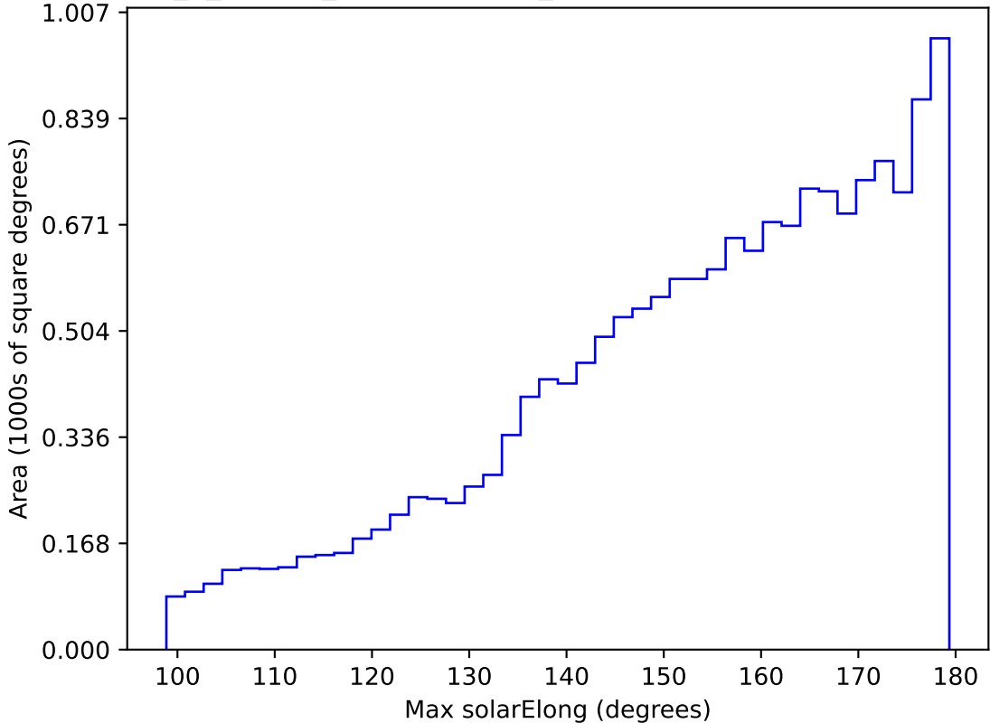
internal_u_expt38_nscale1.5v3.4_10yrs WFD r band: Max solarElong
