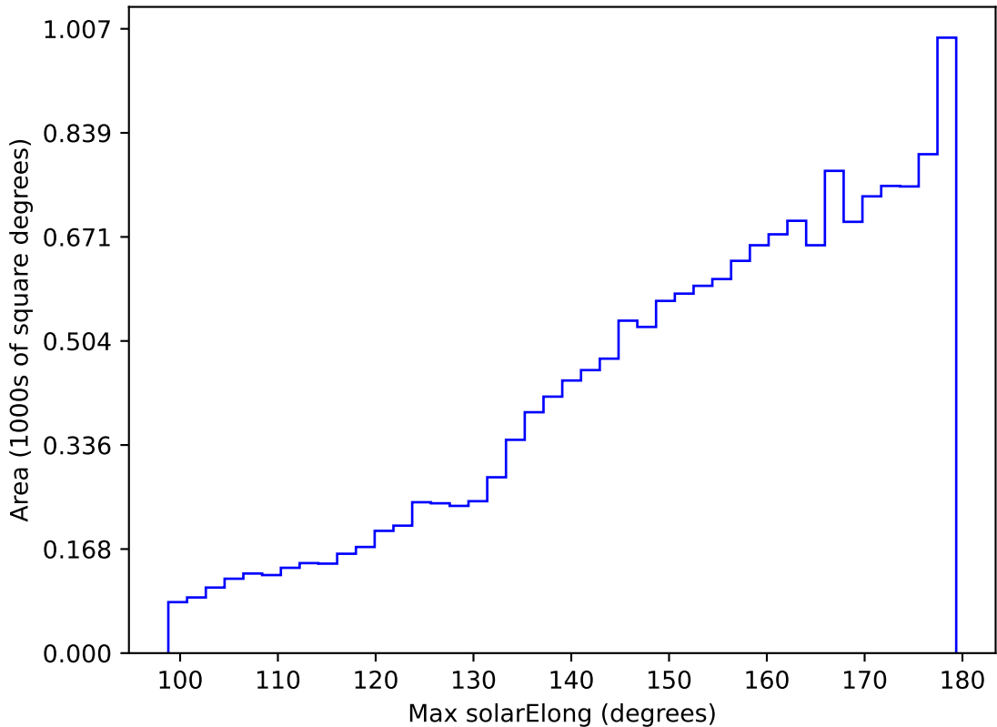
internal_u_expt38_nscale1.5v3.4_10yrs WFD i band: Max solarElong
