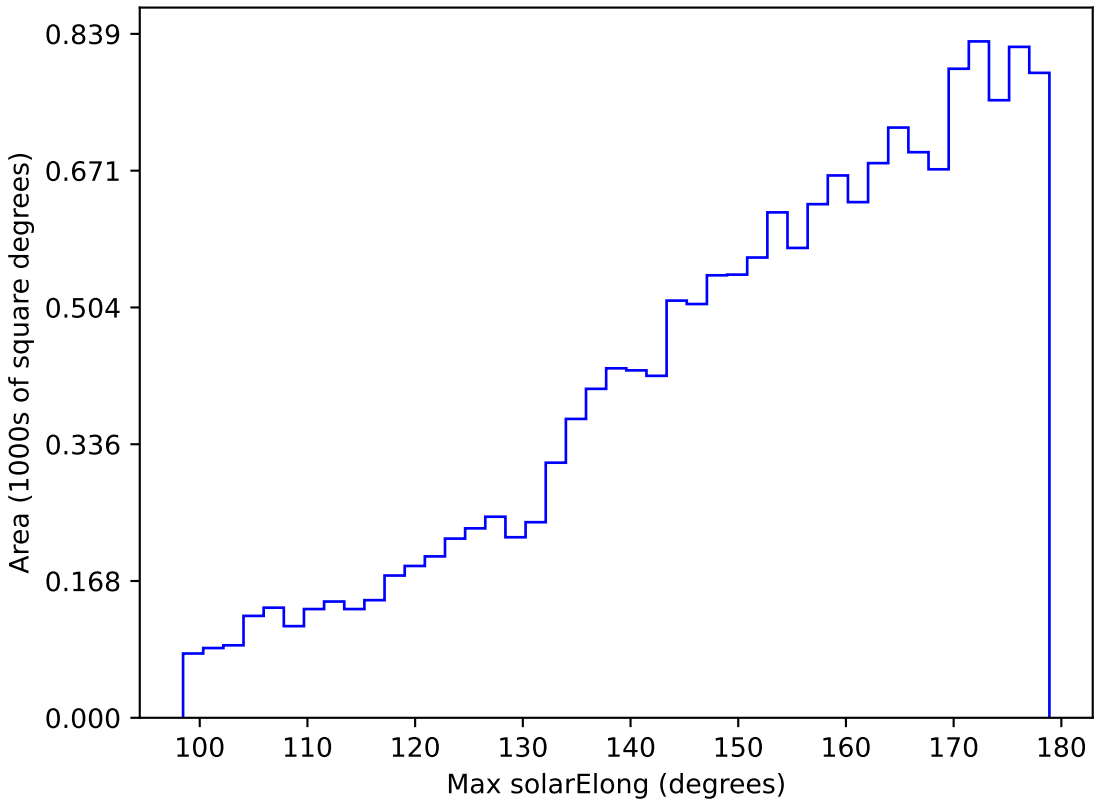
internal_u_expt38_nscale1.5v3.4_10yrs WFD g band: Max solarElong
