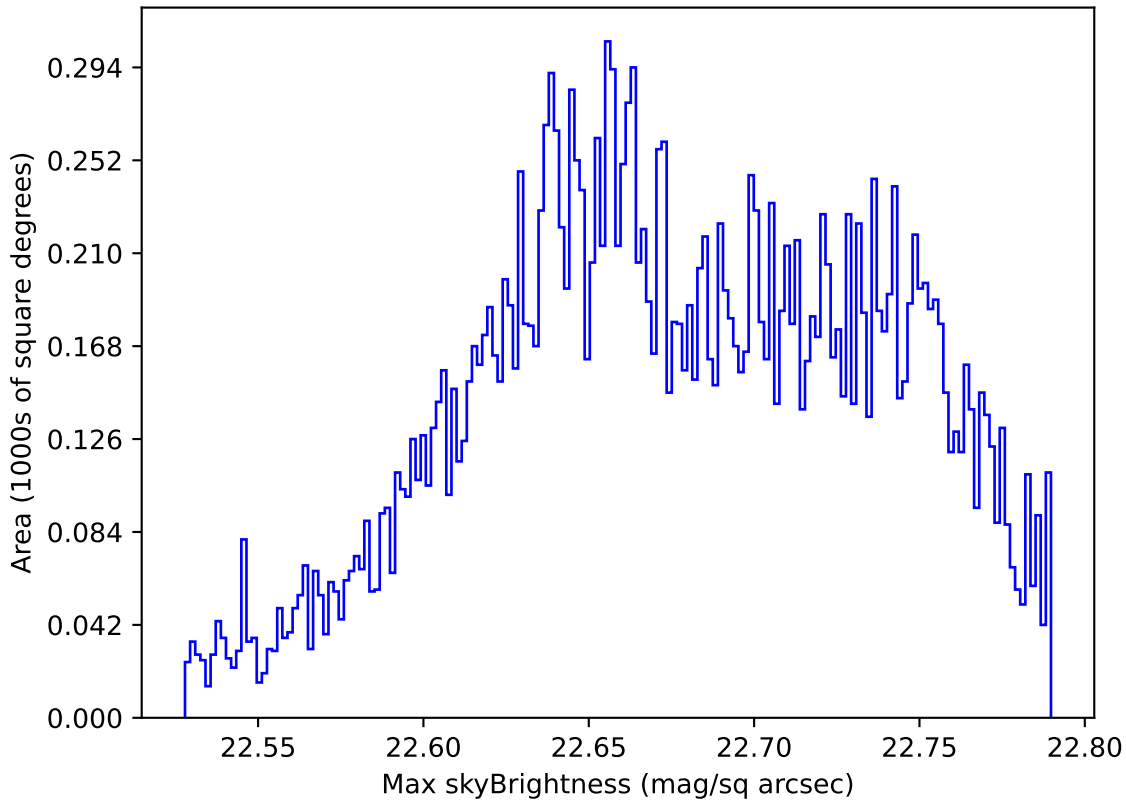
internal_u_expt38_nscale1.5v3.4_10yrs Yr 1 u band: Max skyBrightness
