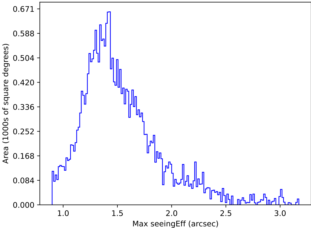
internal_u_expt38_nscale1.5v3.4_10yrs Yr 1 i band: Max seeingEff
