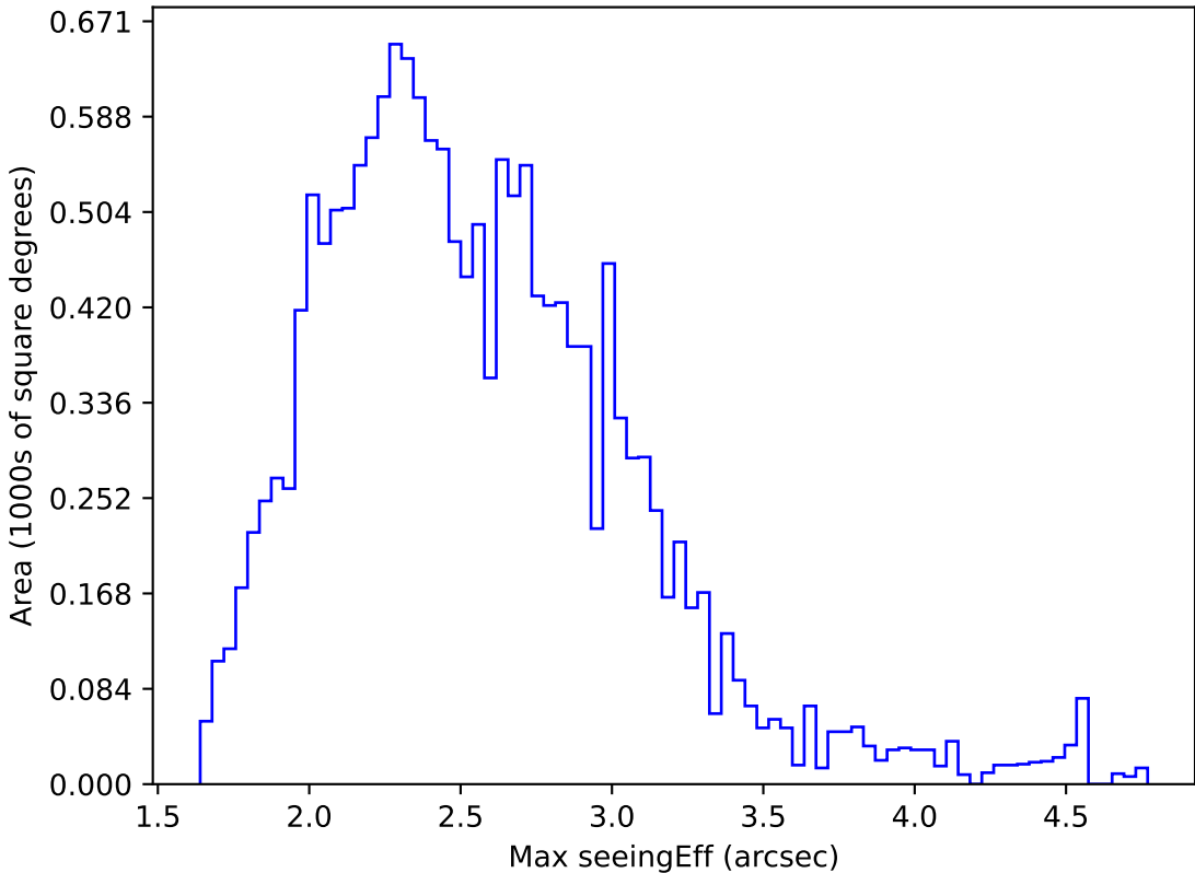
internal_u_expt38_nscale1.5v3.4_10yrs WFD z band: Max seeingEff
