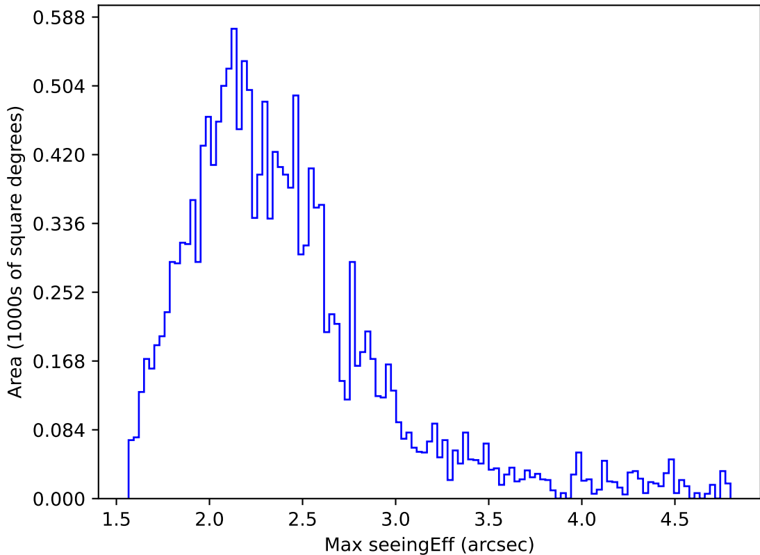
internal_u_expt38_nscale1.5v3.4_10yrs WFD y band: Max seeingEff
