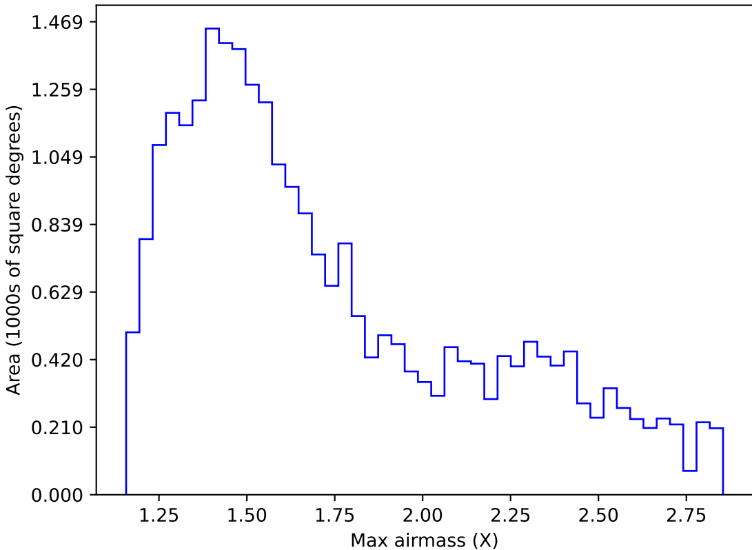
internal_u_expt38_nscale1.5v3.4_10yrs Yr 1 z band: Max airmass
