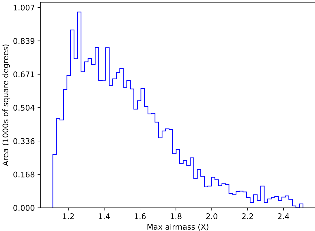
internal_u_expt38_nscale1.5v3.4_10yrs Yr 1 u band: Max airmass
