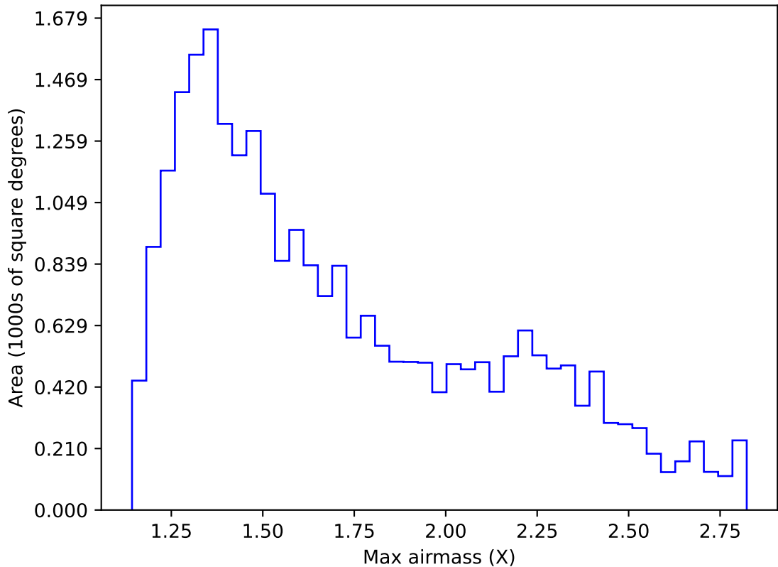
internal_u_expt38_nscale1.5v3.4_10yrs Yr 1 i band: Max airmass
