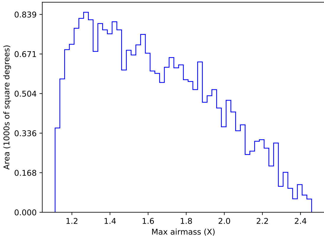
internal_u_expt38_nscale1.5v3.4_10yrs Yr 1 g band: Max airmass
