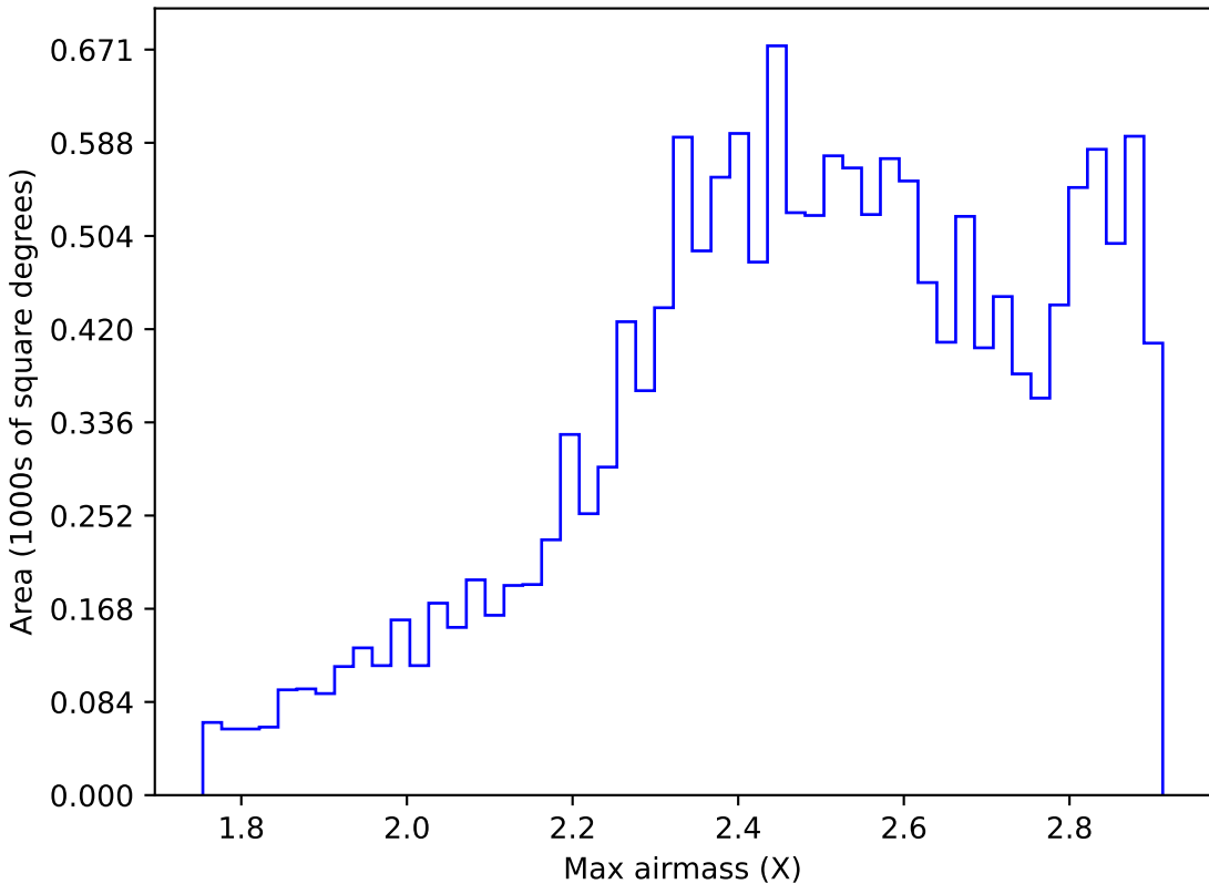
internal_u_expt38_nscale1.5v3.4_10yrs WFD z band: Max airmass
