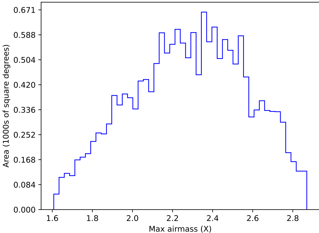
internal_u_expt38_nscale1.5v3.4_10yrs WFD y band: Max airmass
