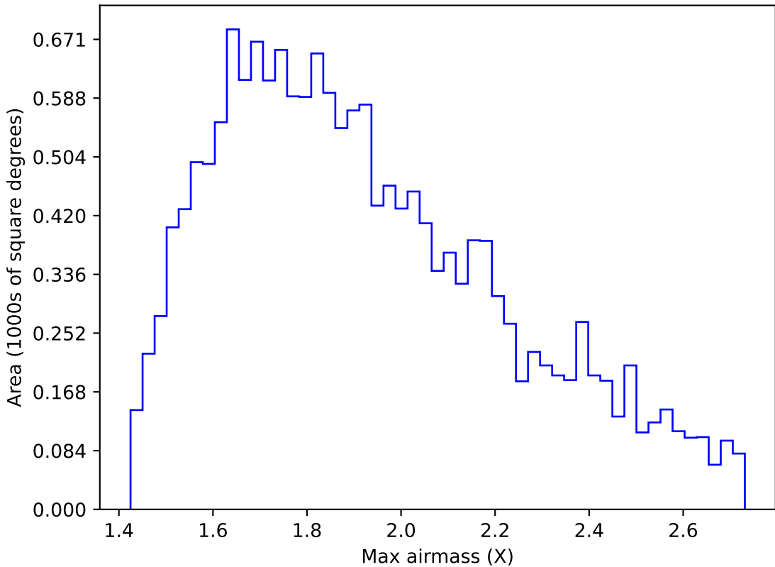
internal_u_expt38_nscale1.5v3.4_10yrs WFD u band: Max airmass
