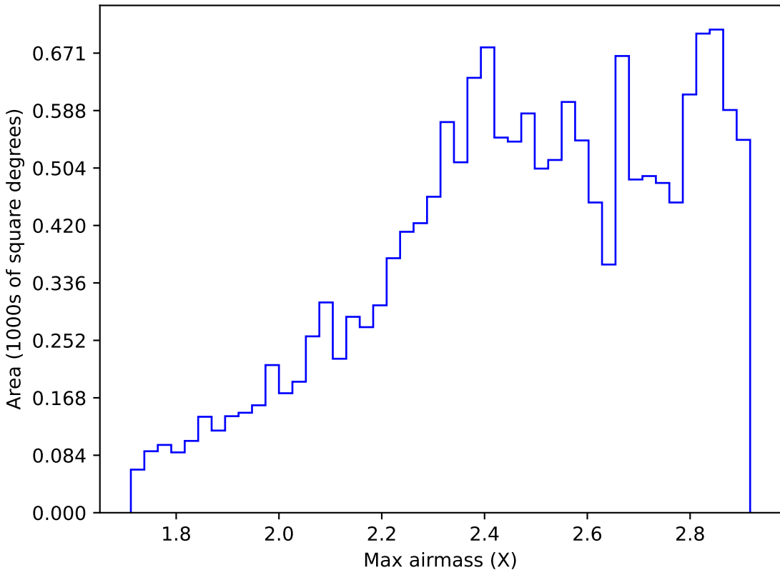
internal_u_expt38_nscale1.5v3.4_10yrs WFD i band: Max airmass
