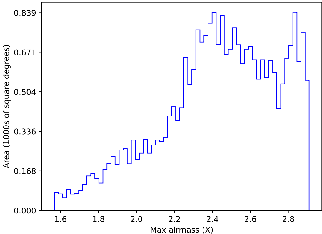
internal_u_expt38_nscale1.5v3.4_10yrs All sky z band: Max airmass
