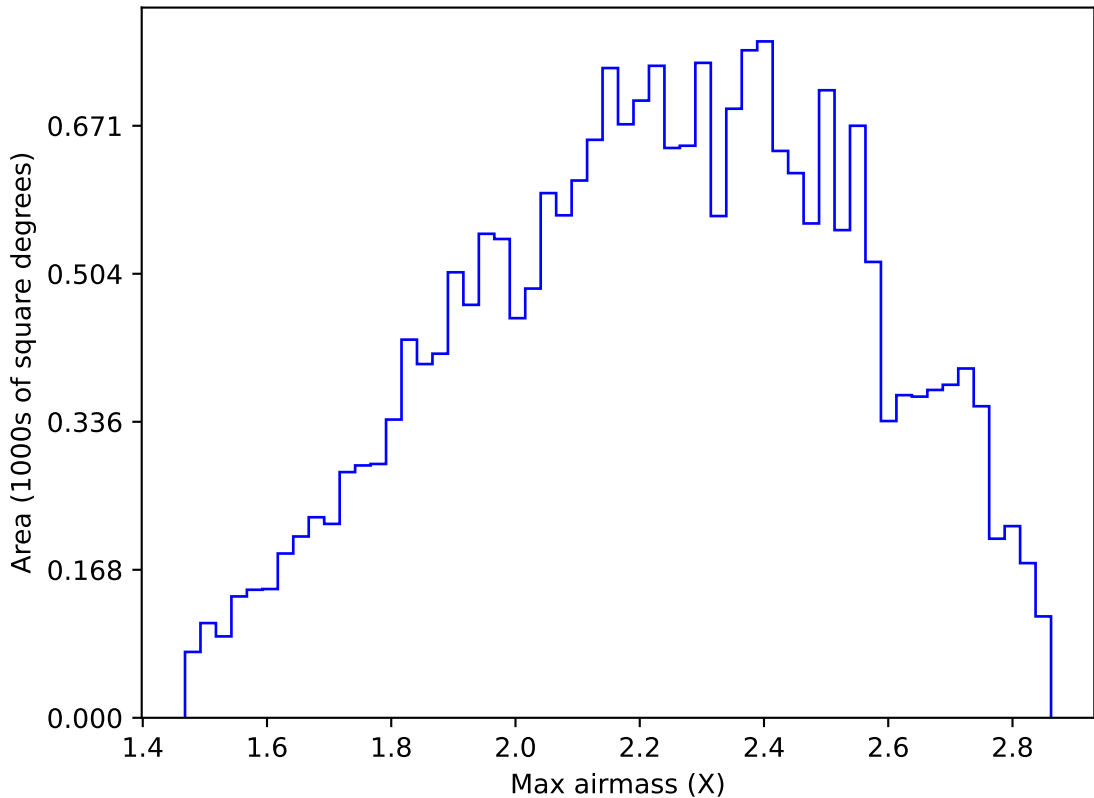
internal_u_expt38_nscale1.5v3.4_10yrs All sky y band: Max airmass
