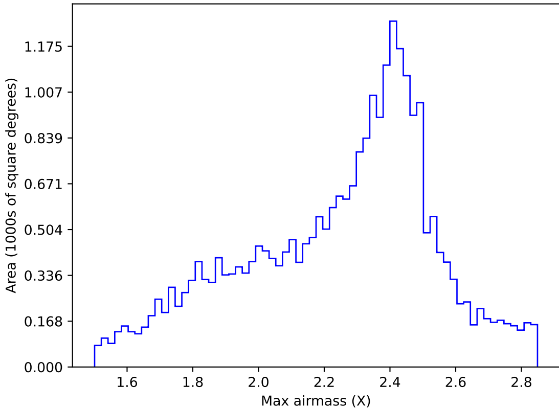
internal_u_expt38_nscale1.5v3.4_10yrs All sky r band: Max airmass
