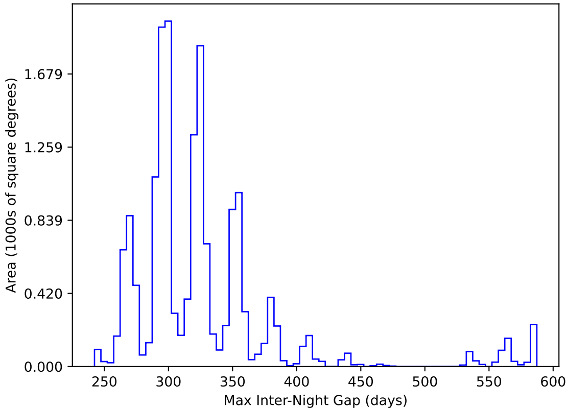
internal_u_expt38_nscale1.5v3.4_10yrs WFD y band: Max Inter-Night Gap
