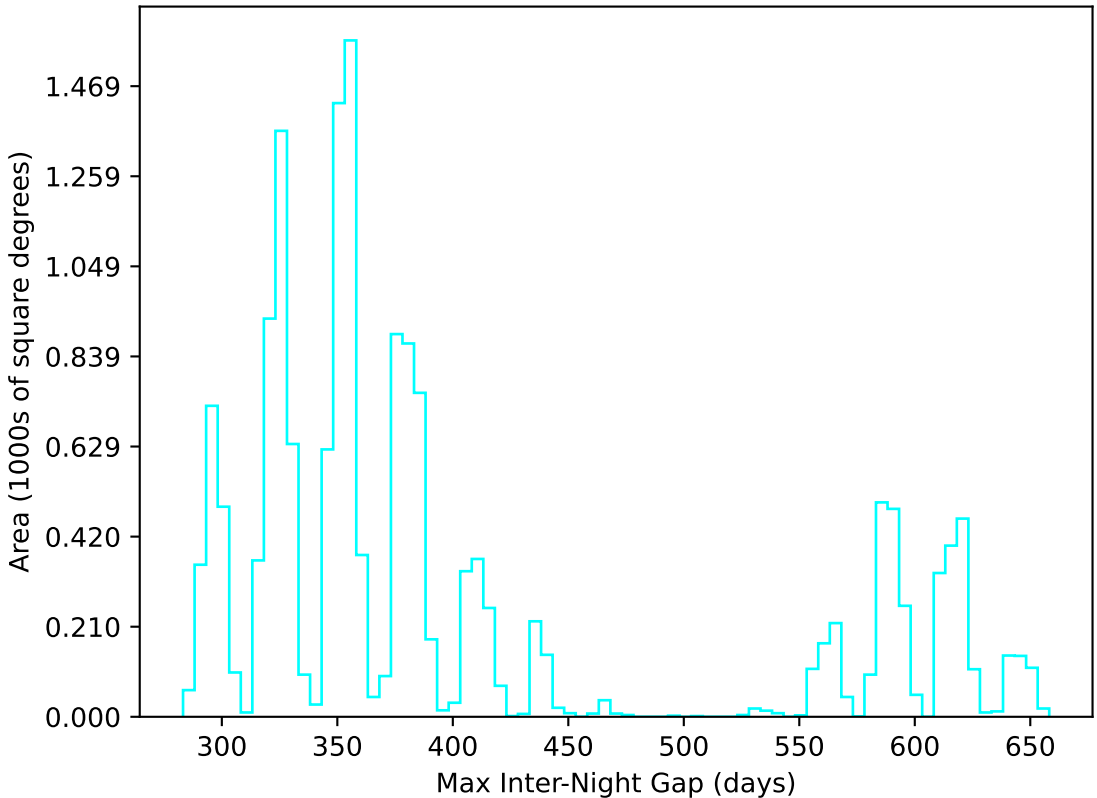
internal_u_expt38_nscale1.5v3.4_10yrs WFD u band: Max Inter-Night Gap
