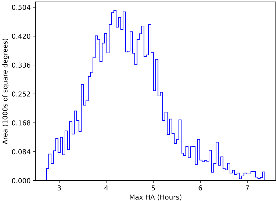
internal_u_expt38_nscale1.5v3.4_10yrs WFD r band: Max HA
