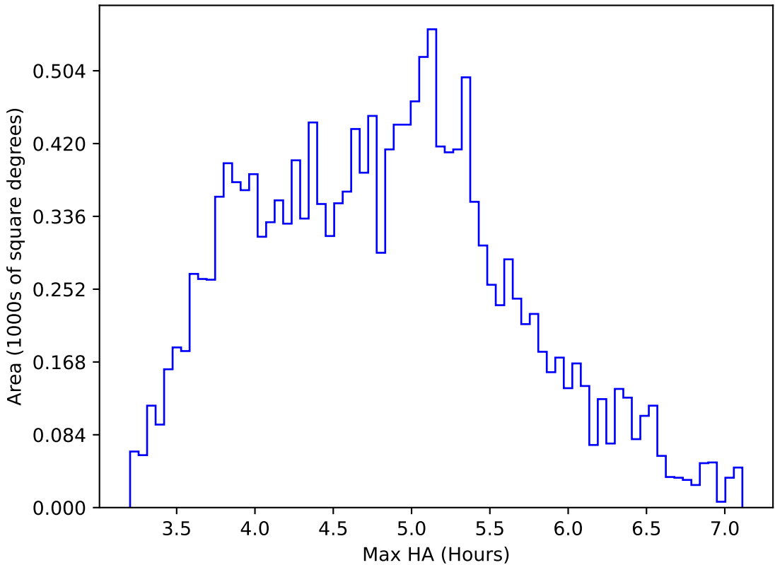
internal_u_expt38_nscale1.5v3.4_10yrs WFD i band: Max HA
