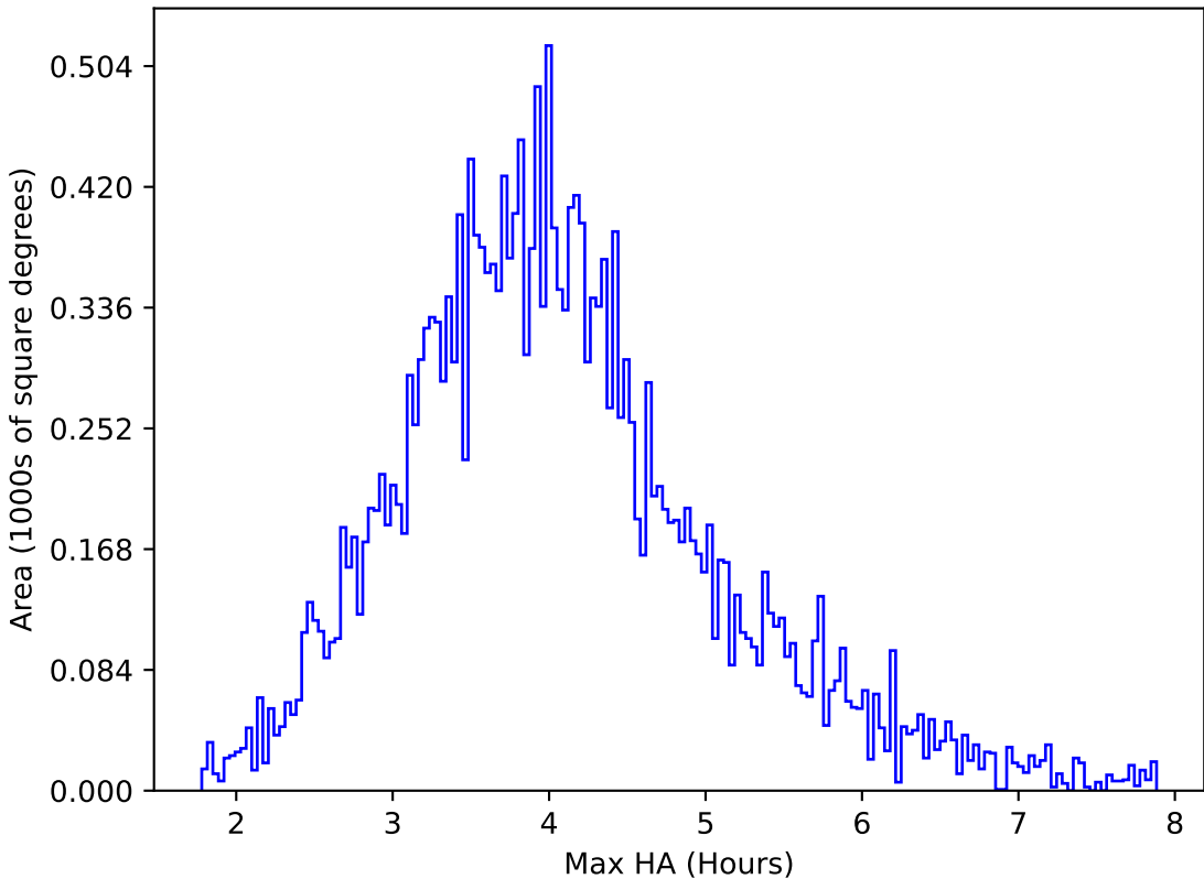
internal_u_expt38_nscale1.5v3.4_10yrs All sky u band: Max HA
