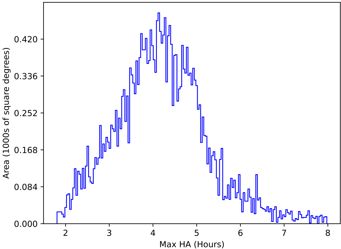
internal_u_expt38_nscale1.5v3.4_10yrs All sky r band: Max HA
