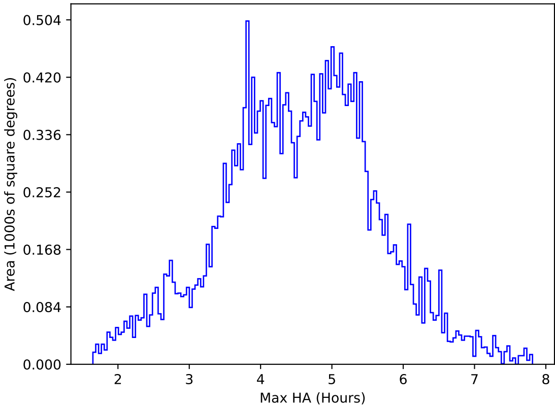
internal_u_expt38_nscale1.5v3.4_10yrs All sky i band: Max HA
