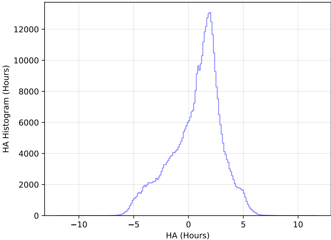
internal_u_expt38_nscale1.5v3.4_10yrs WFD z band: HA Histogram
