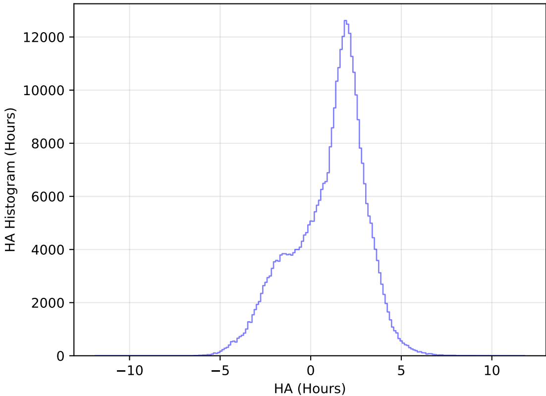
internal_u_expt38_nscale1.5v3.4_10yrs WFD y band: HA Histogram
