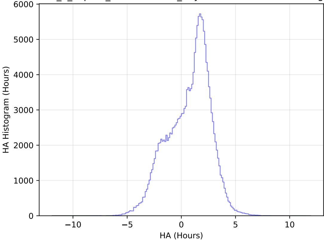
internal_u_expt38_nscale1.5v3.4_10yrs WFD u band: HA Histogram
