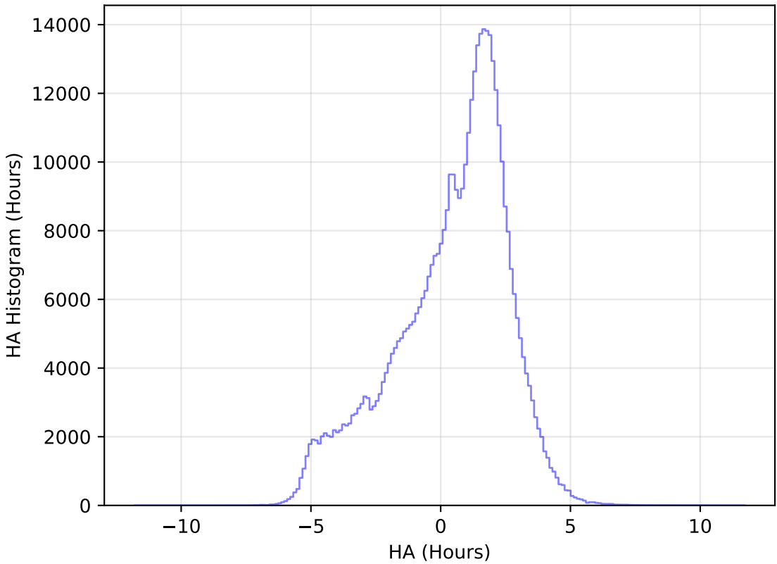
internal_u_expt38_nscale1.5v3.4_10yrs WFD r band: HA Histogram
