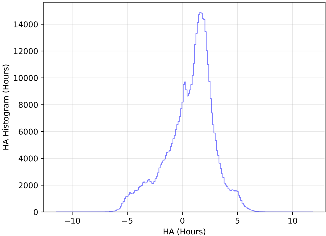
internal_u_expt38_nscale1.5v3.4_10yrs WFD i band: HA Histogram
