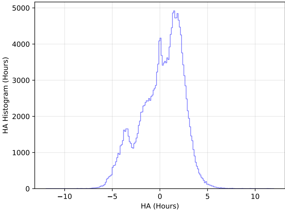
internal_u_expt38_nscale1.5v3.4_10yrs WFD g band: HA Histogram
