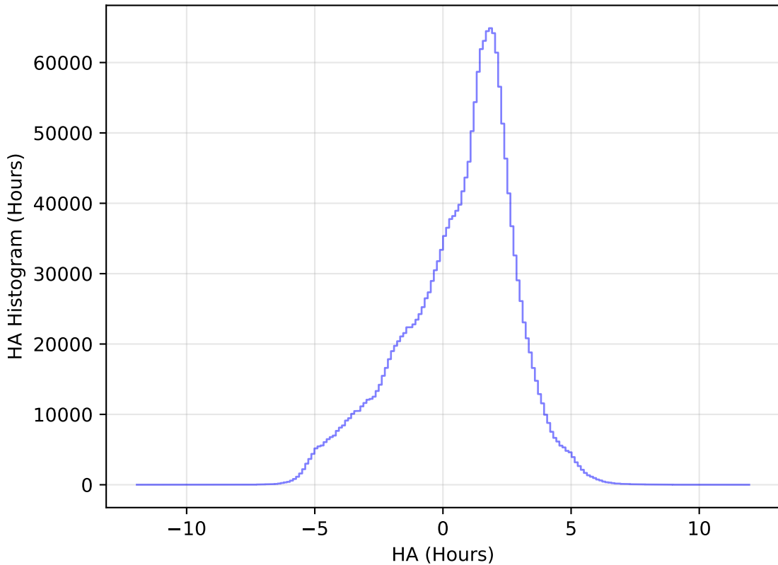
internal_u_expt38_nscale1.5v3.4_10yrs WFD all bands: HA Histogram
