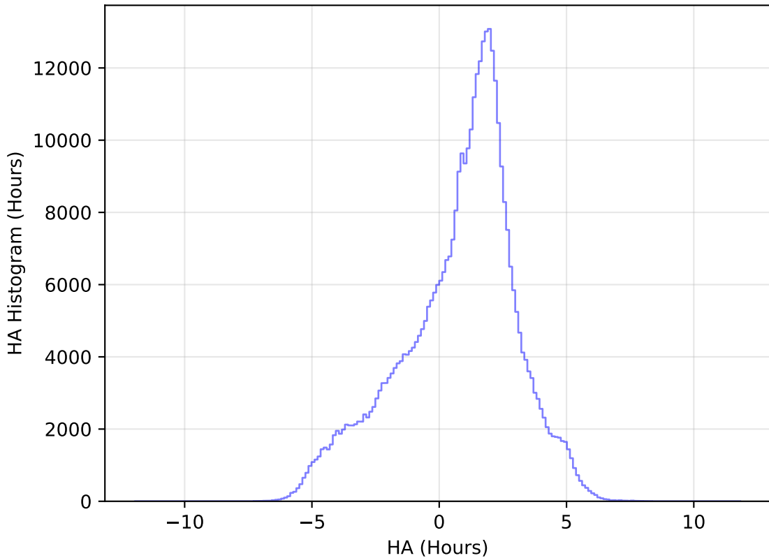
internal_u_expt38_nscale1.5v3.4_10yrs All sky z band: HA Histogram
