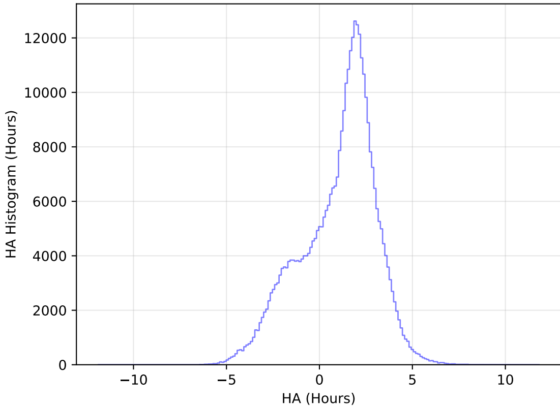
internal_u_expt38_nscale1.5v3.4_10yrs All sky y band: HA Histogram
