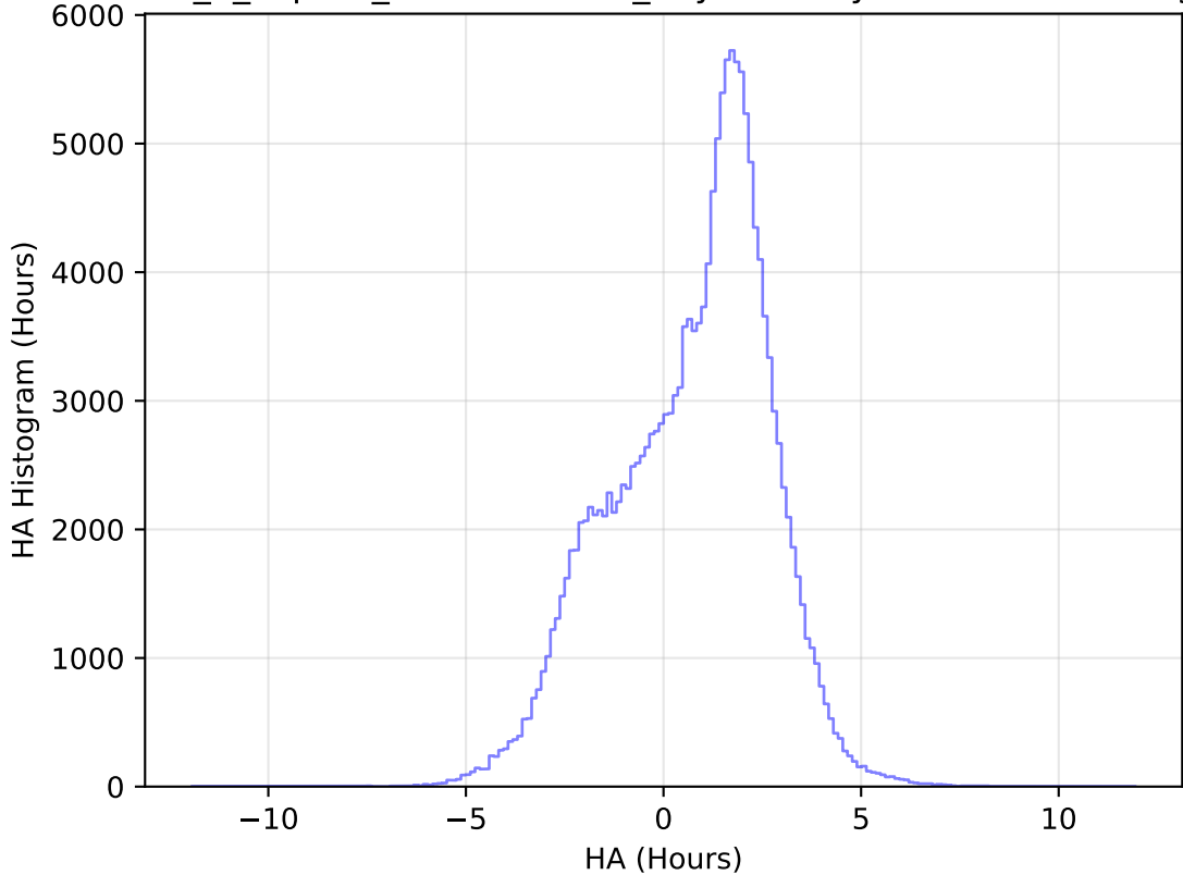
internal_u_expt38_nscale1.5v3.4_10yrs All sky u band: HA Histogram
