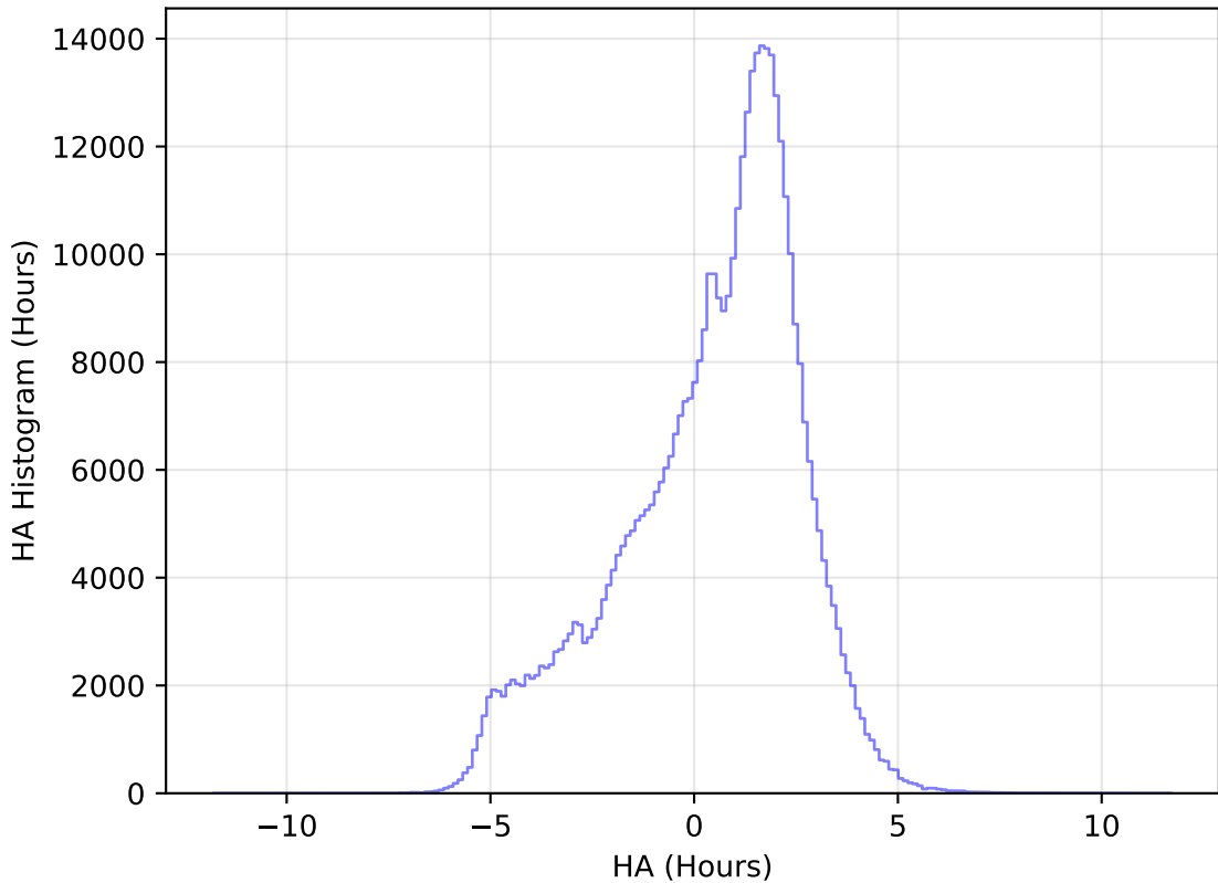
internal_u_expt38_nscale1.5v3.4_10yrs All sky r band: HA Histogram
