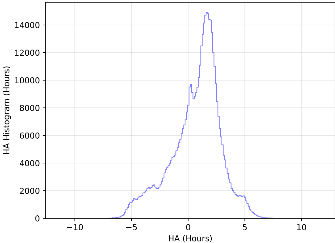
internal_u_expt38_nscale1.5v3.4_10yrs All sky i band: HA Histogram
