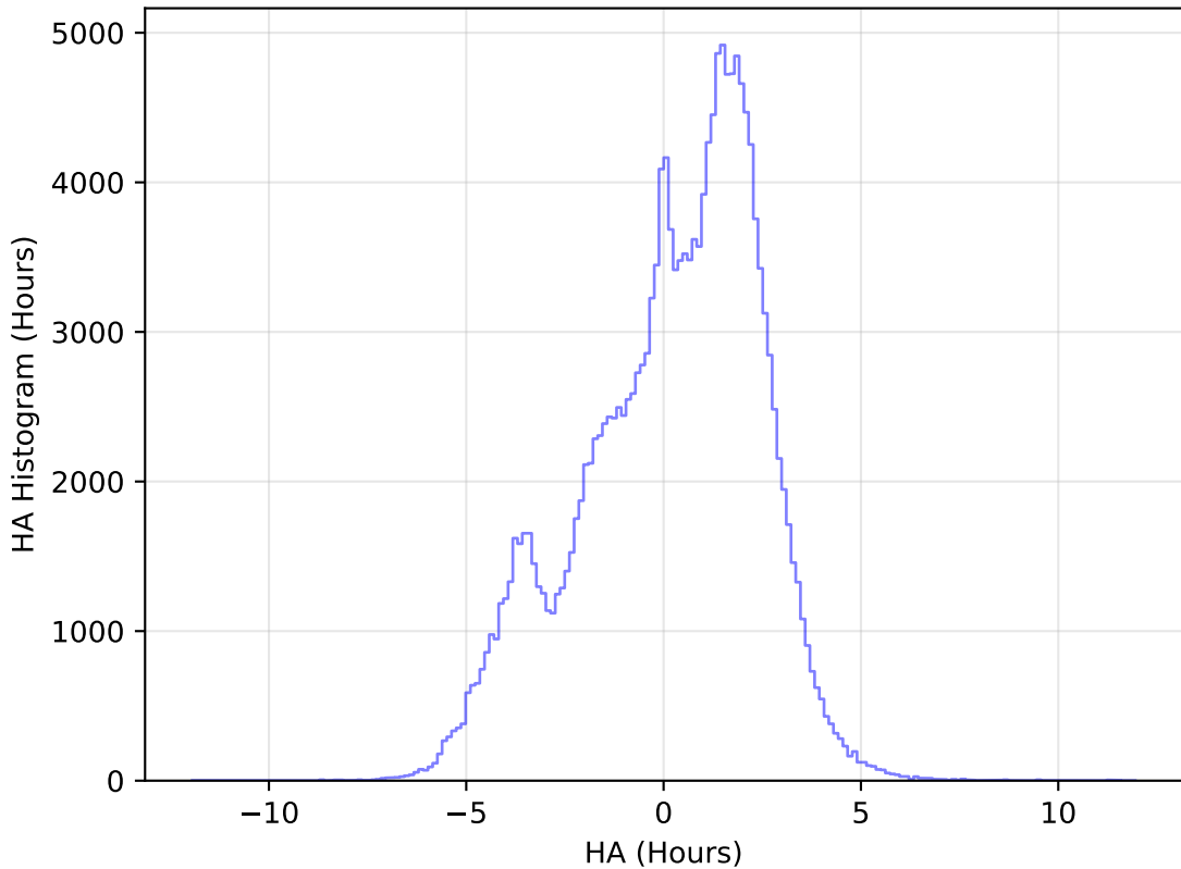
internal_u_expt38_nscale1.5v3.4_10yrs All sky g band: HA Histogram
