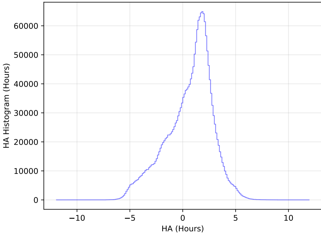
internal_u_expt38_nscale1.5v3.4_10yrs All sky all bands: HA Histogram
