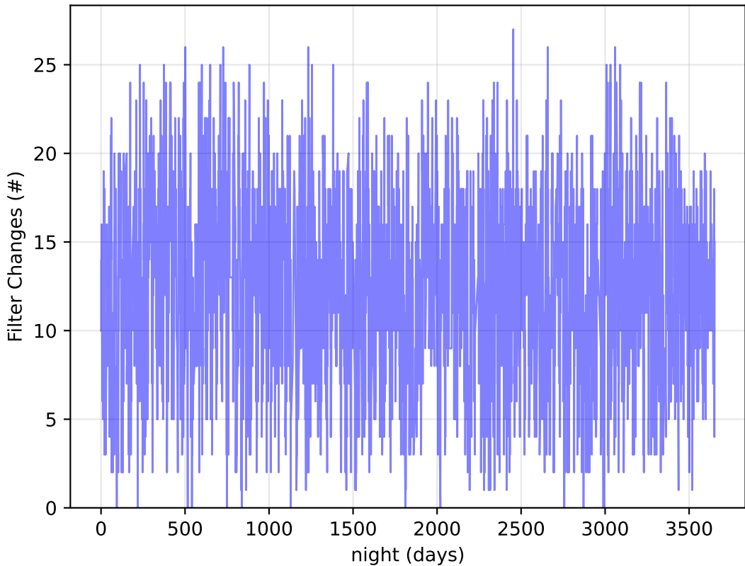
internal_u_expt38_nscale1.5v3.4_10yrs Per Night: Filter Changes
