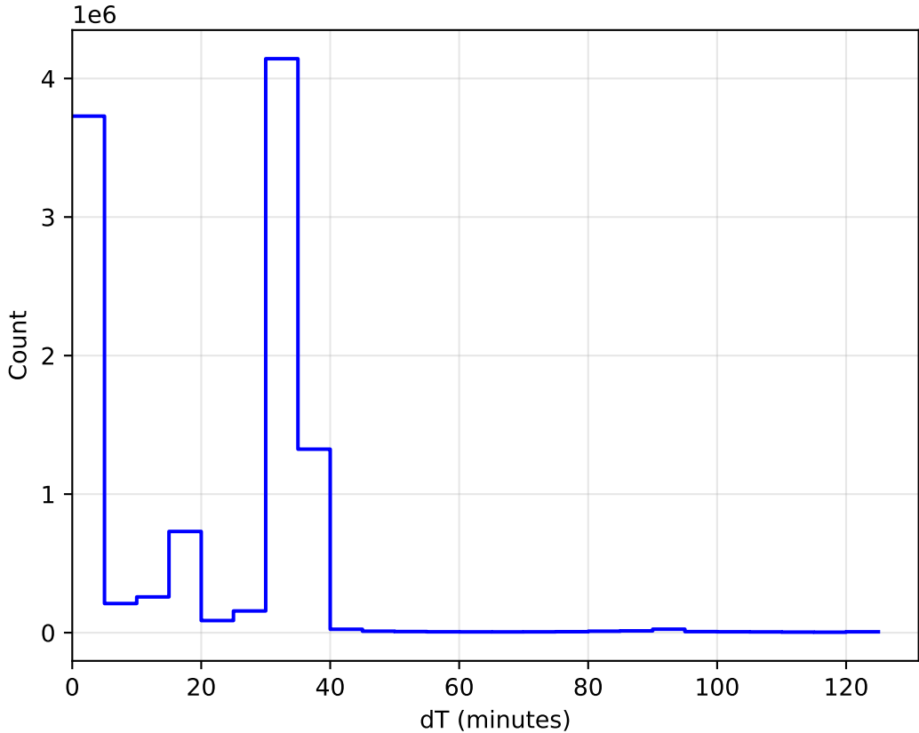
internal_u_expt38_nscale1.5v3.4_10yrs WFD: DeltaT Histogram
