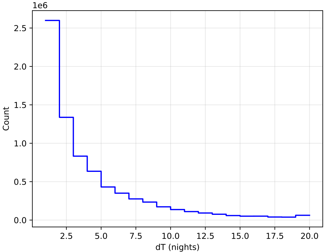
internal_u_expt38_nscale1.5v3.4_10yrs WFD all bands: DeltaNight Histogram
