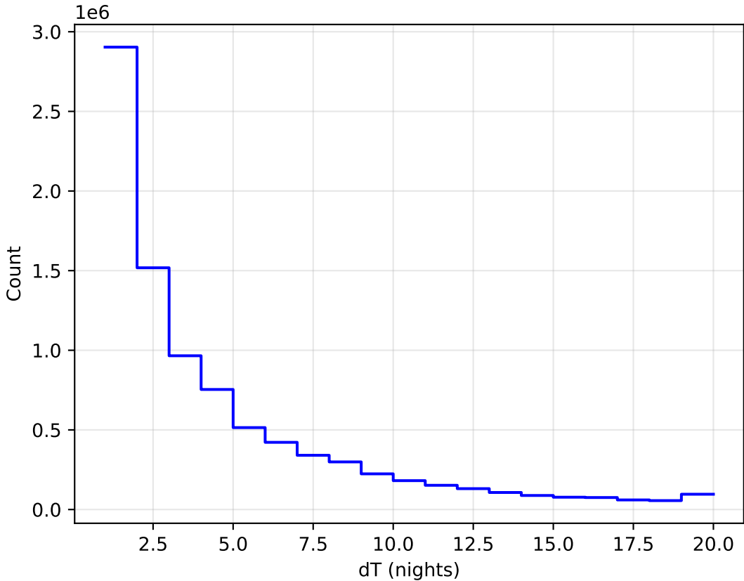
internal_u_expt38_nscale1.5v3.4_10yrs All sky all bands: DeltaNight Histogram
