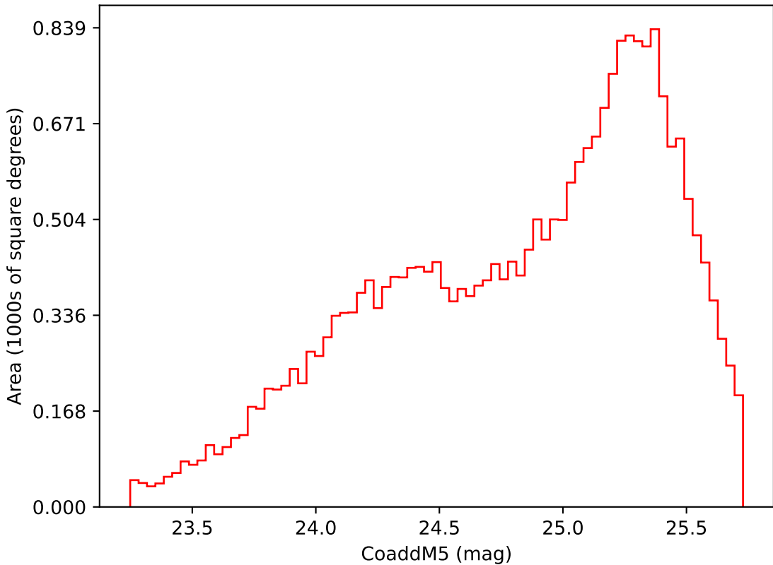
internal_u_expt38_nscale1.5v3.4_10yrs Yr 3-4 i band: CoaddM5
