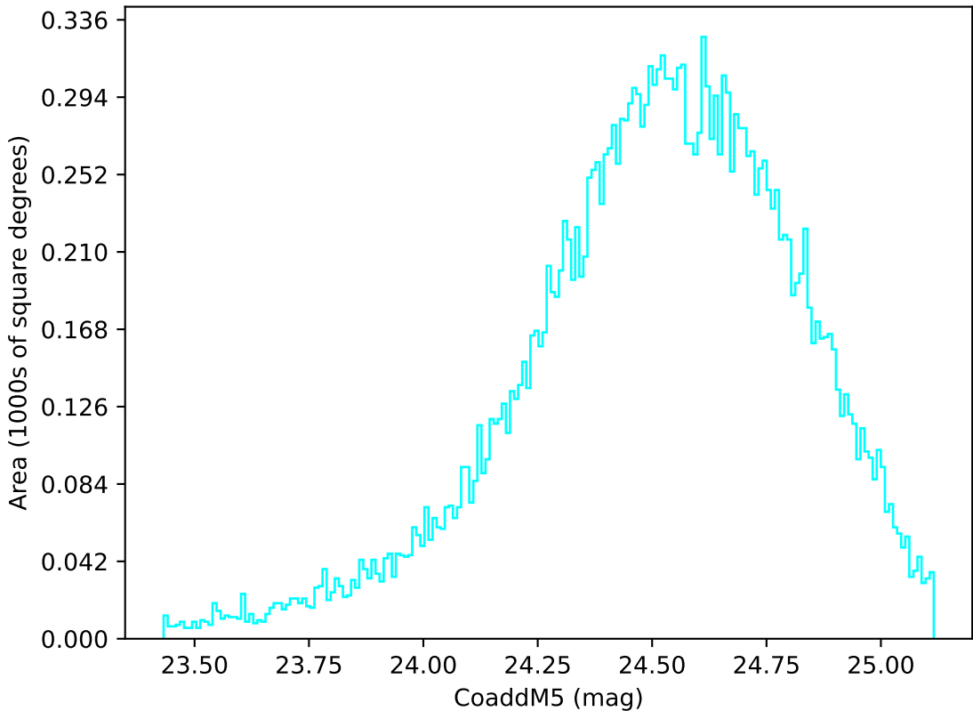
internal_u_expt38_nscale1.5v3.4_10yrs Yr 1 u band: CoaddM5
