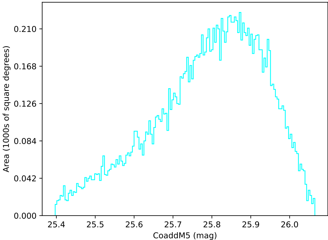
internal_u_expt38_nscale1.5v3.4_10yrs WFD u band: CoaddM5
