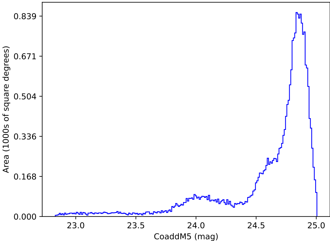
internal_u_expt38_nscale1.5v3.4_10yrs All sky y band: CoaddM5
