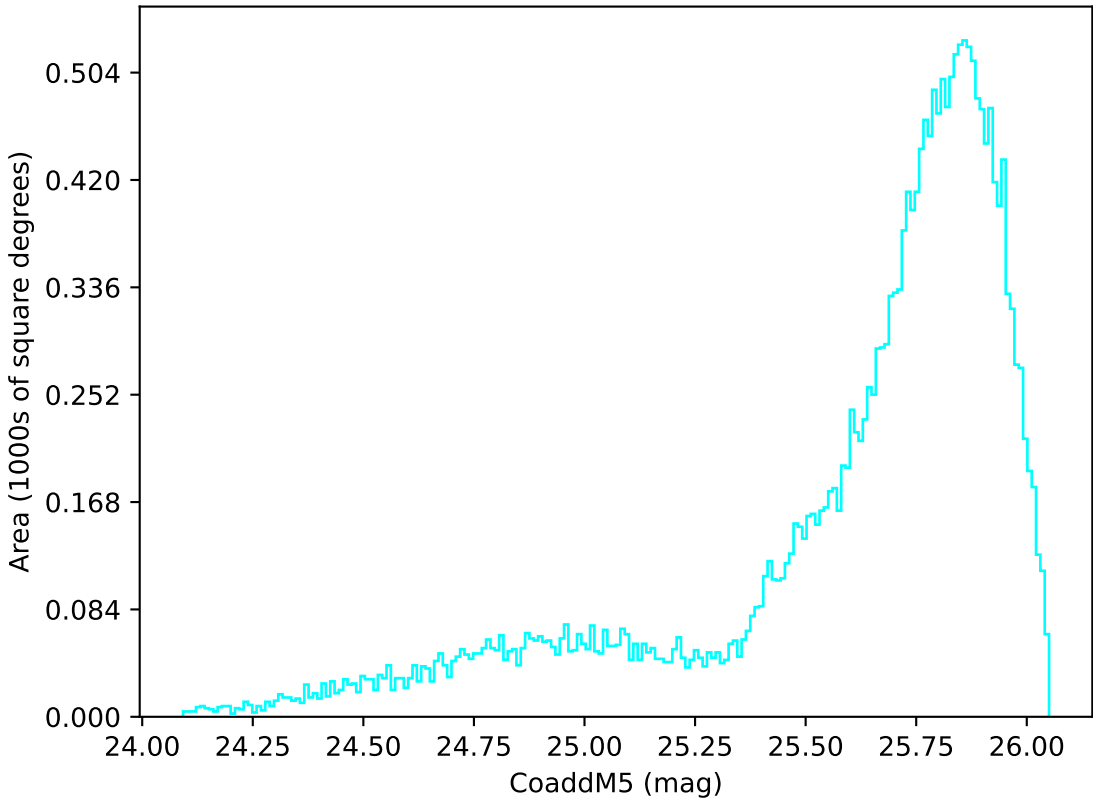
internal_u_expt38_nscale1.5v3.4_10yrs All sky u band: CoaddM5
