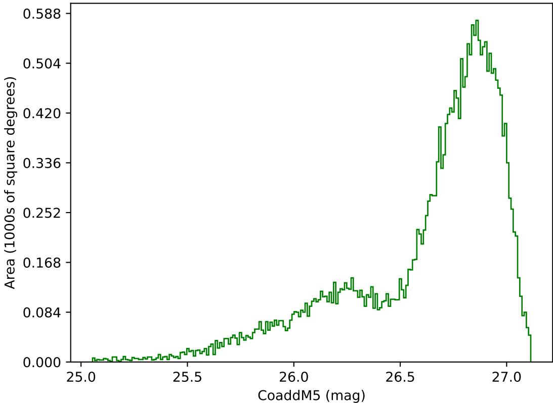
internal_u_expt38_nscale1.5v3.4_10yrs All sky g band: CoaddM5
