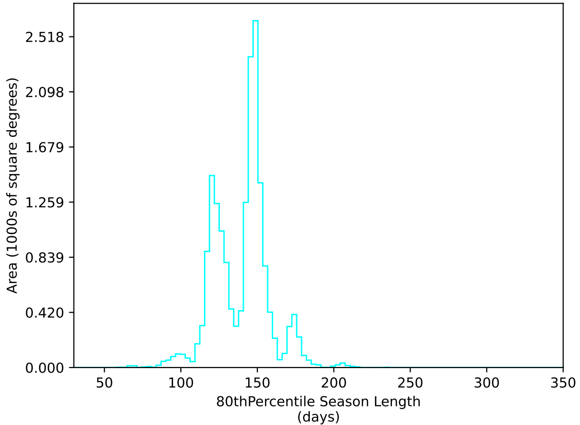
internal_u_expt38_nscale1.5v3.4_10yrs WFD u band: 80thPercentile Season Length
